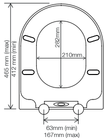
Max/min fixing adjustment
